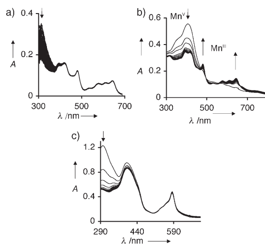
Figure 2. Time-resolved diode-array absorption spectra (25 °C) recorded at a) 3-ms intervals (0–0.3 s) during the reaction of 1 -Mn (40 μM) with peroxyxynitrite (1400 μM) at pH 7.4; b) at 20-s intervals (0–200 s) during the slow transformation of the (oxo)manganese(V) complex 1 -Mn(O) to 1 -Mn at pH 7.4; and c) at 10-s intervals (0–110 s) during the reaction of 1 -Mn (36 μM) with peroxyxynitrite (720 μM) at pH 12.7. Note: the spectrum of independently prepared 1 -Mn(O) is identical to that obtained by the reaction of 1 -Mn with peroxyxynitrite at the same pH value.
