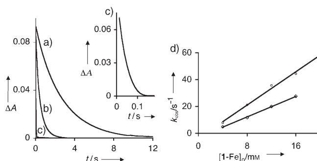
Figure 1. a–c) Decomposition of 385 \mu\text{M} peroxynitrite at pH 7.4 and 25 °C monitored at \lambda = 302 nm, the \lambda_{\text{max}} of peroxynitrite, without catalyst (a), or in the presence of 16 \mu\text{M} (4 mol %) 1-Mn (b) or 1-Fe (c; shown at two timescales). d) Observed decomposition rates of peroxynitrite (385 \mu\text{M} , pH 7.4) as a function of 1-Fe concentration at 25 °C (lower trace) and 37 °C (upper trace).
