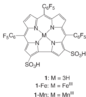
Scheme 1. Amphiphilic corrole 1 and its metal complexes.
