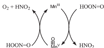
Scheme 2. Proposed catalytic cycle for disproportionation of peroxyxynitrite catalyzed by manganese(III) corrole.
